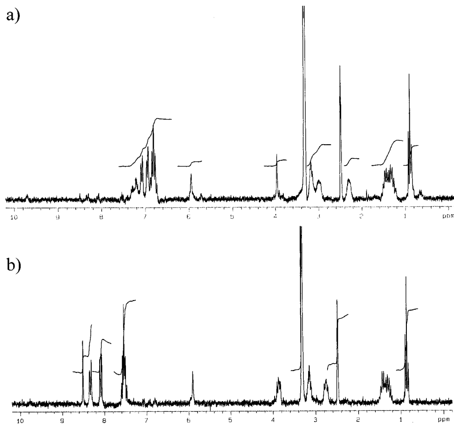
Fig. Thermal change of ^1\text{H} NMR spectrum of 2 in \text{DMSO-d}_6 a) at 22^\circ\text{C} and b) after 15 min at 150^\circ\text{C} .
